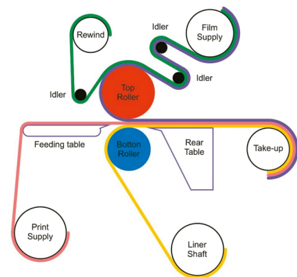
Threading Diagram
